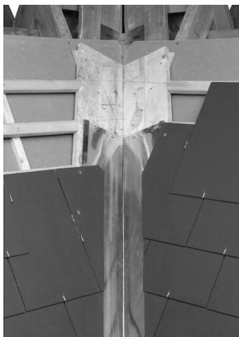
Open ki[e]lgoot
