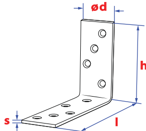
Frame connector
