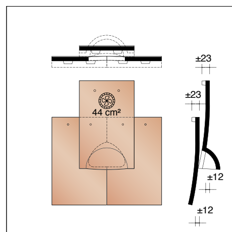
KSHI/KGOX 8611 Kit de ventilation - 44 cm 2
